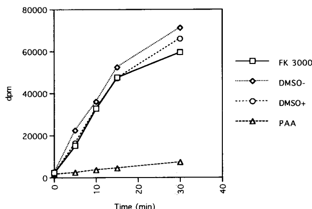
Fig. 6. Effect of FK 3000 on the activity of HSV DNA polymerase. Effects of FK 3000 (500 \mu g/ml, open square) and PAA (120 \mu g/ml, open triangle) on HSV DNA polymerase activity were examined in the reaction mixture as described in the text. The reaction mixture with 1 % DMSO (DMSO+) or without DMSO (DMSO-) was used as negative controls. 21)
