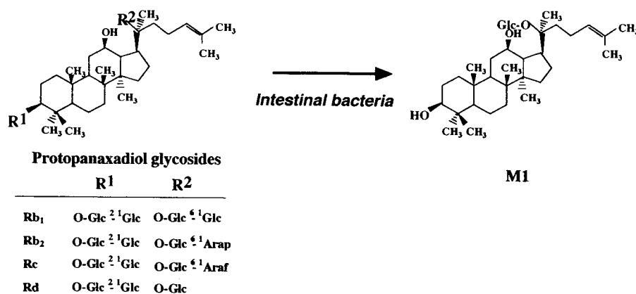
Fig. 1 Structure of protopanaxadiol glycosides and their metabolic compound M1.
