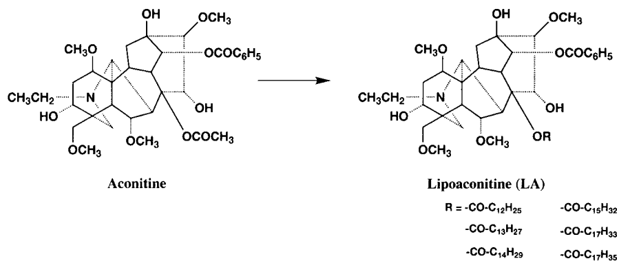
Chart 1. Conversion of aconitine to lipoaconitine by B. fragilis .
