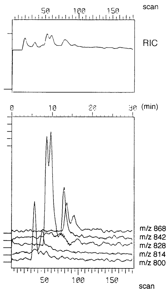
Fig. 1 Frit-FAB LC/MS chromatogram of LA formed after incubation of aconitine with B. fragilis . Column, Nucleosil 5CN (25 cm \times 4.6 mm i.d.); mobile phase, CH 3 CN-H 2 O-AcOH-glycerol (50:50:1:0.5); flow rate, 0.8 ml/min; FAB energy, 4 kV; detection, positive ion mode.
