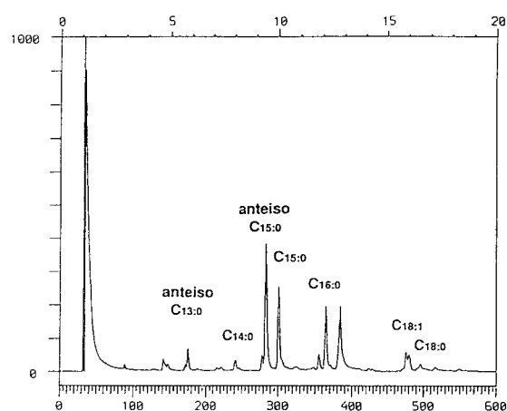
Fig. 2 GC/MS ion chromatogram of the fatty acid methyl esters of LA formed after incubation of aconitine with B. fragilis . Column, silicone OV-101 (30 m × 0.25 mm i.d.); column temperature, 150–250°C, 4°C/min; carrier gas, He (50 ml/min); inlet mode, split; ionization voltage, 70 eV.
