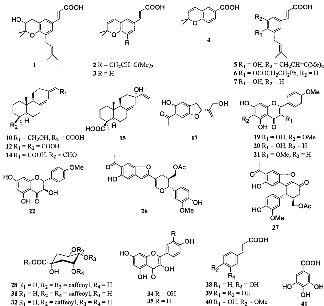
Fig. 1 Structure of the compounds detected in B. dracunculifolia .
