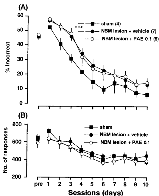
Fig. 2 Effect of paeoniflorin (0.1 mg/kg/day) on brightness discrimination learning in rats with unilateral NBM lesion. Paeoniflorin (PAE : 0.1 mg/kg) was administered perorally 90 min before daily training sessions. The number of animals used are shown in parenthesis. Each data points represents the mean \pm S.E.M. The % incorrect data obtained in the early phase (from day 1 to day 5) were statistically analyzed. *** P < 0.001 compared with sham-operated group.
